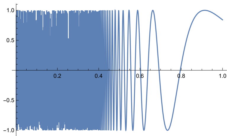
图 1.6: \alpha = 0, \beta < 0
