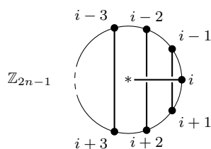
Figure 7.2: Blocks in the parallel class \mathcal{D}_i
